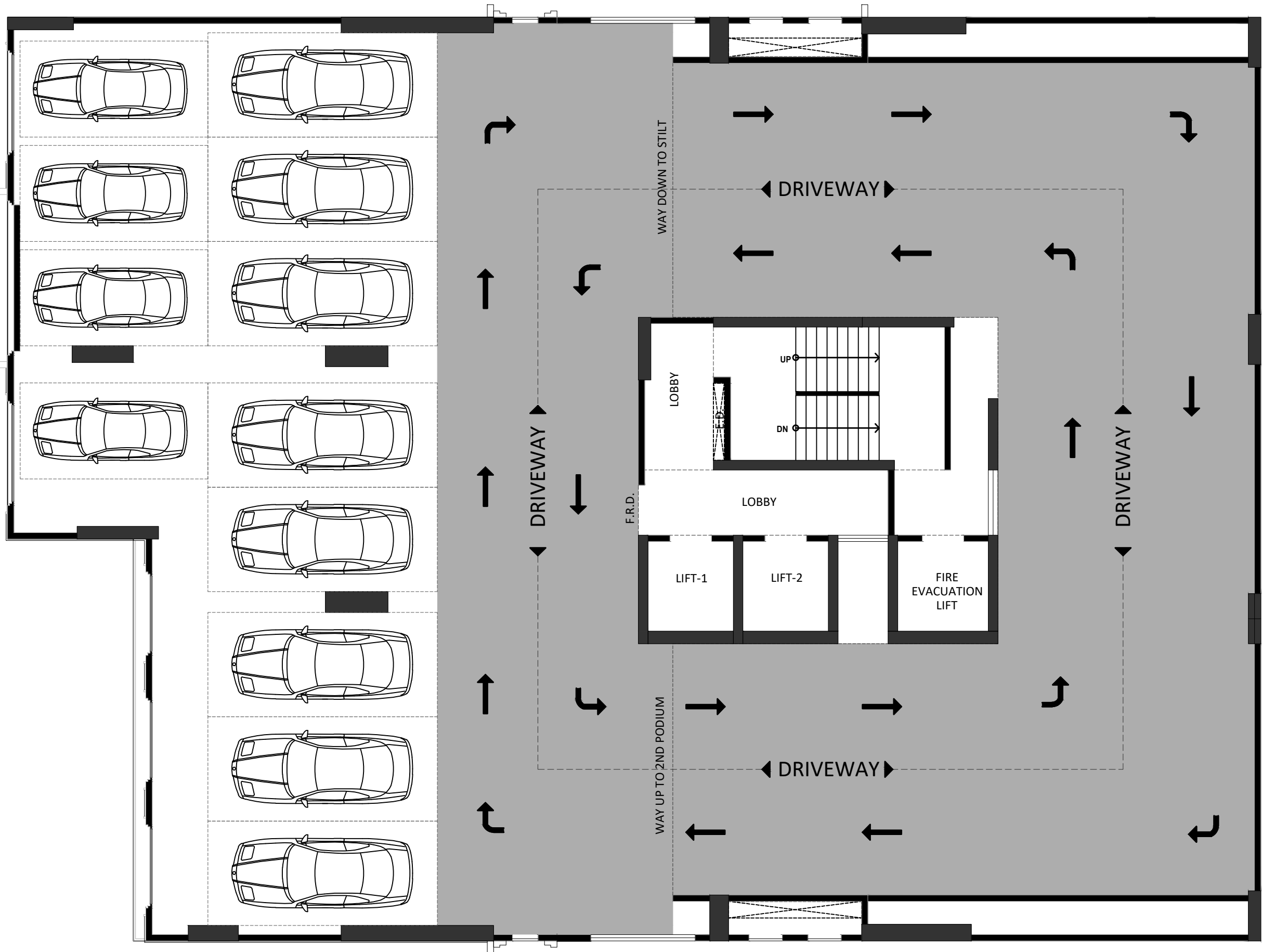
1ST TO 3RD PODIUM FLOOR PLAN
