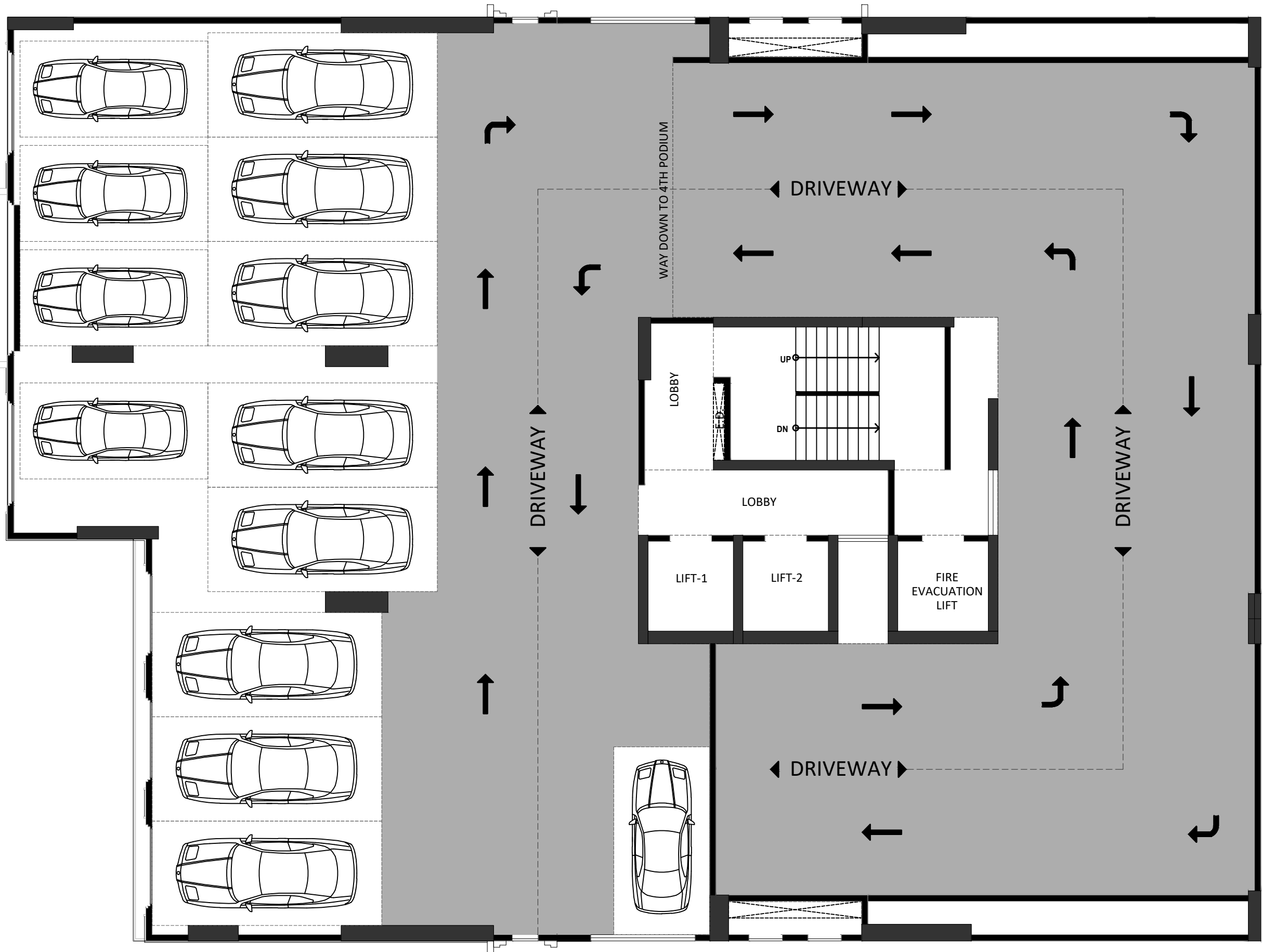
4TH PODIUM FLOOR PLAN
